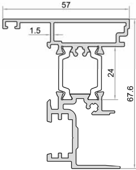
W6-508 AĞIRLIK / WEIGHT (KG/M.) 1,453 (PVC) 1,438 (POL.)
