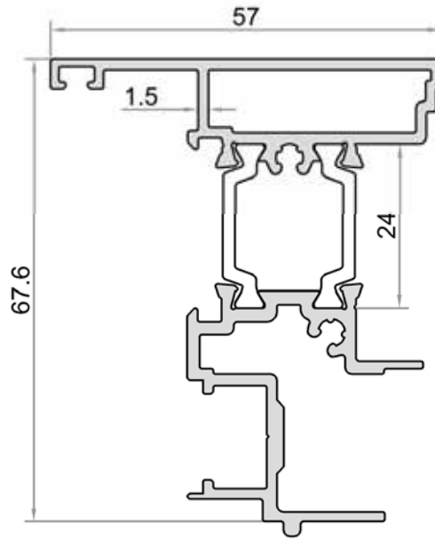
W6-509 AĞIRLIK / WEIGHT (KG/M.) 1,409 (PVC) 1,395 (POL.)
