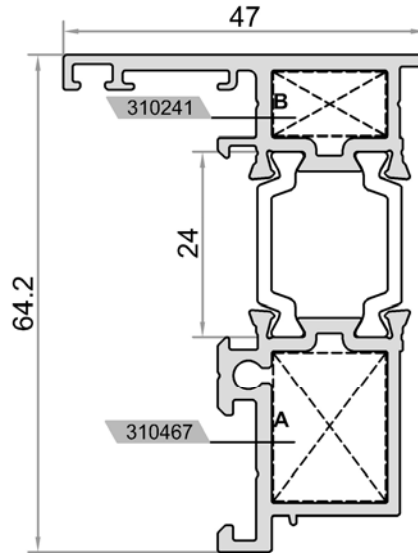
W6-510 VİDALI KÖŞE TAKOZLARI SCREW CORNER CLEATS 310466 (A) 310178 (B) AĞIRLIK / WEIGHT (KG/M.) 1,262 (PVC) 1,247 (POL.)
